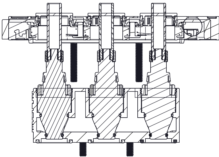
SECTION B-B
